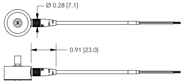
ZCC200 DIMENSIONS WHEN MATED TO SENSORS
