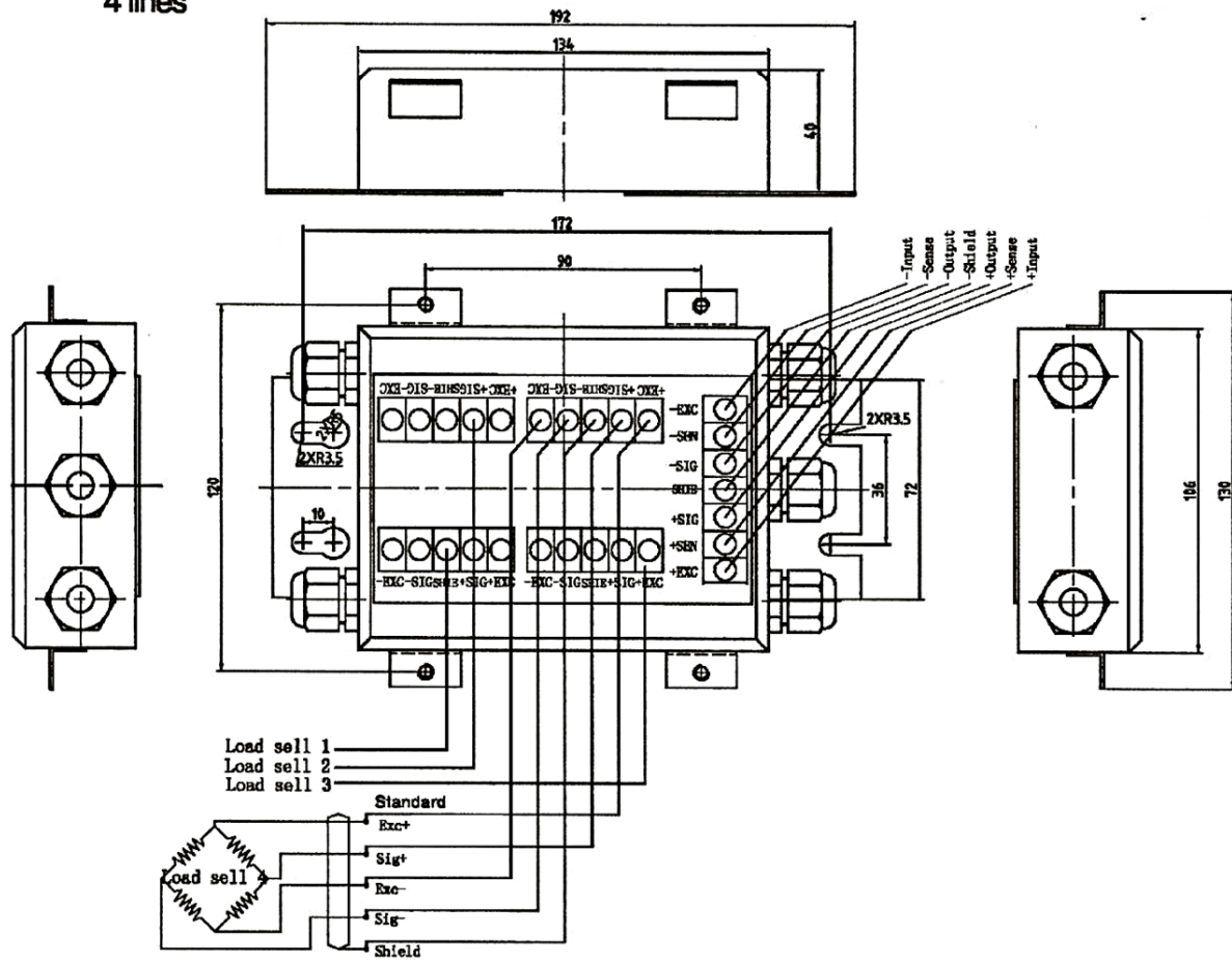
Wiring Schematic Diagram
