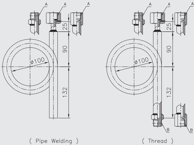
( Pipe Welding )
