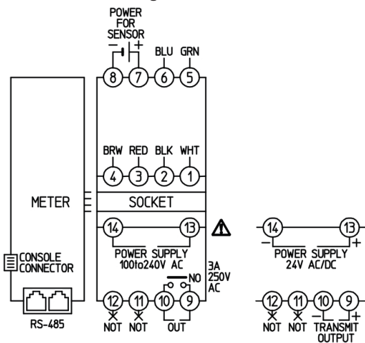
Modular Jack Pin (WIL-101-TU side arrangement)
