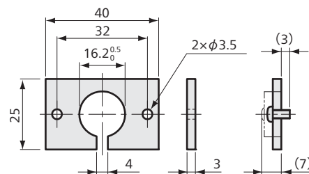
CFM-16B (LMB/LMBT-A-500 to 2KN)
