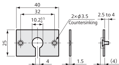
CFM-10B (LMB/LMBT-A-10 to 200N)
