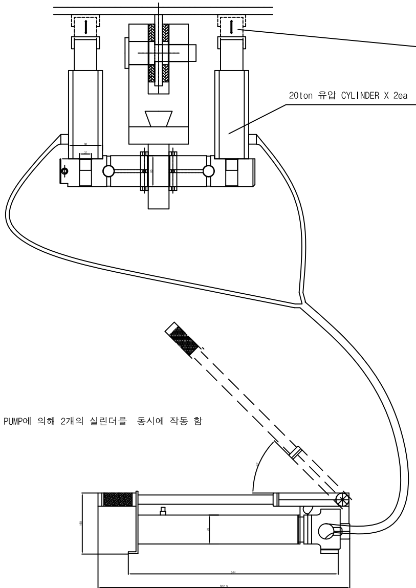
25 TON PEDEYE LOADCELL JIG
